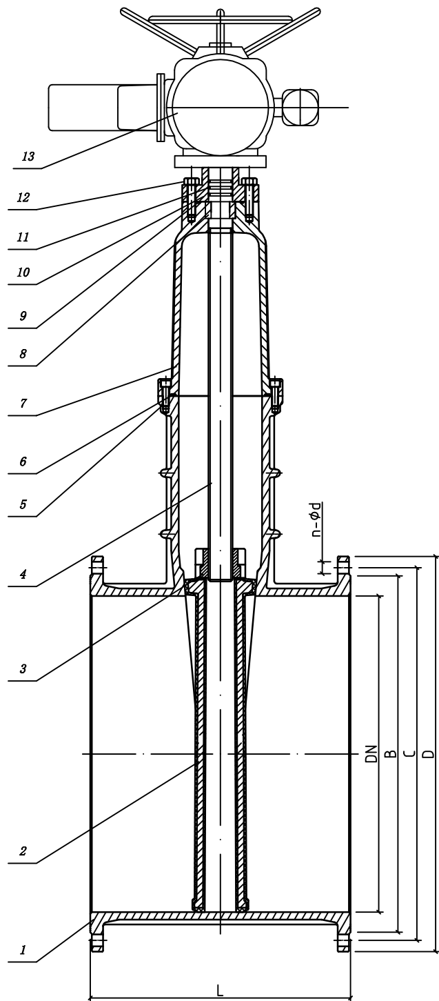
Resilient Seated Gate Valve DIN3352-F4
